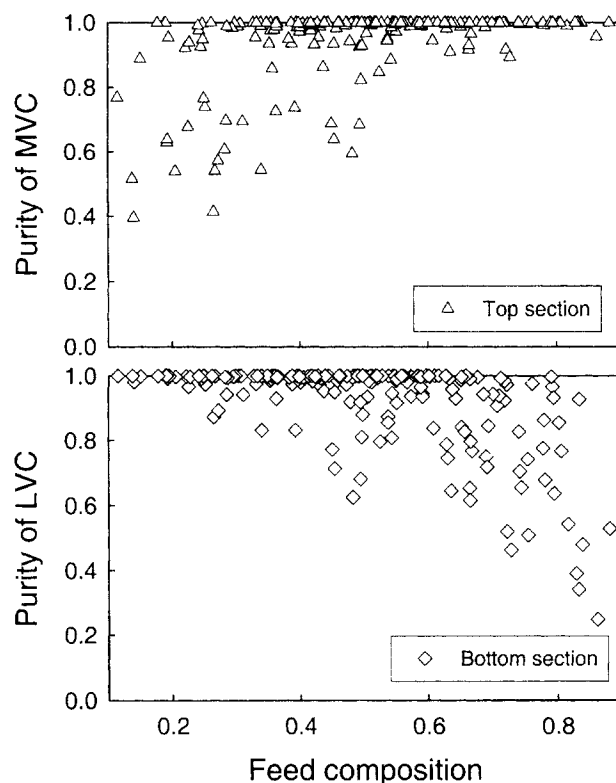
Figure 4. Product purity of the middle-vessel column.
