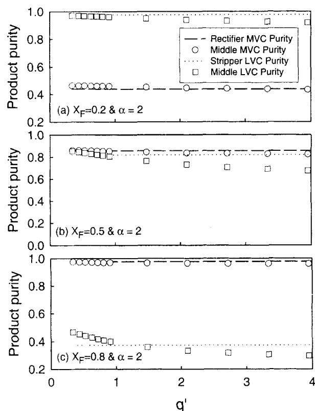
Figure 5. Effect of q' on the product purity of the middle-vessel column ( N = 5 and R = 2 ).
