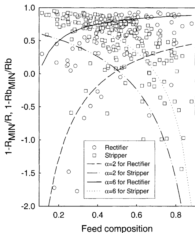
Figure 7. R -Feasibilities of the rectifier and the stripper [for clarity solid lines at fixed conditions ( N = 5 , R = 2 ) are added].
