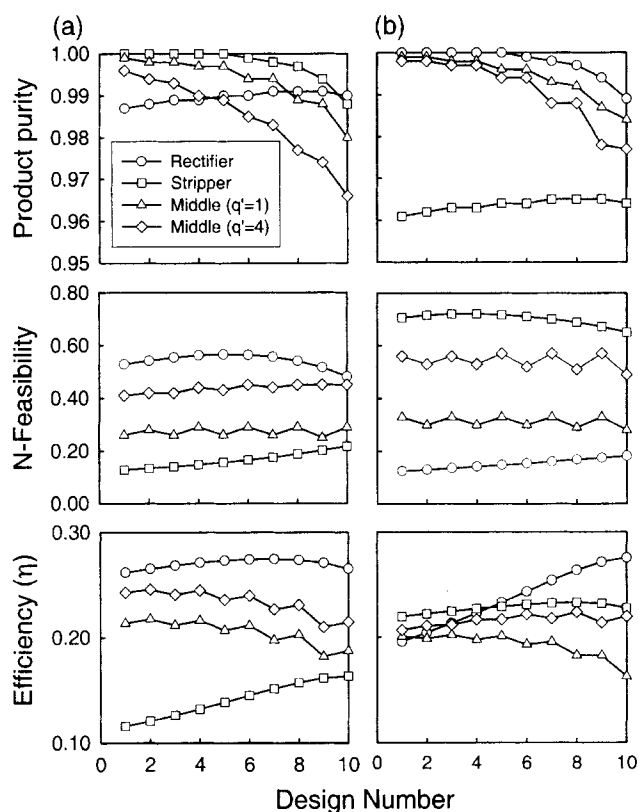
Figure 13. Trends of multiobjective functions with respect to case numbers.
